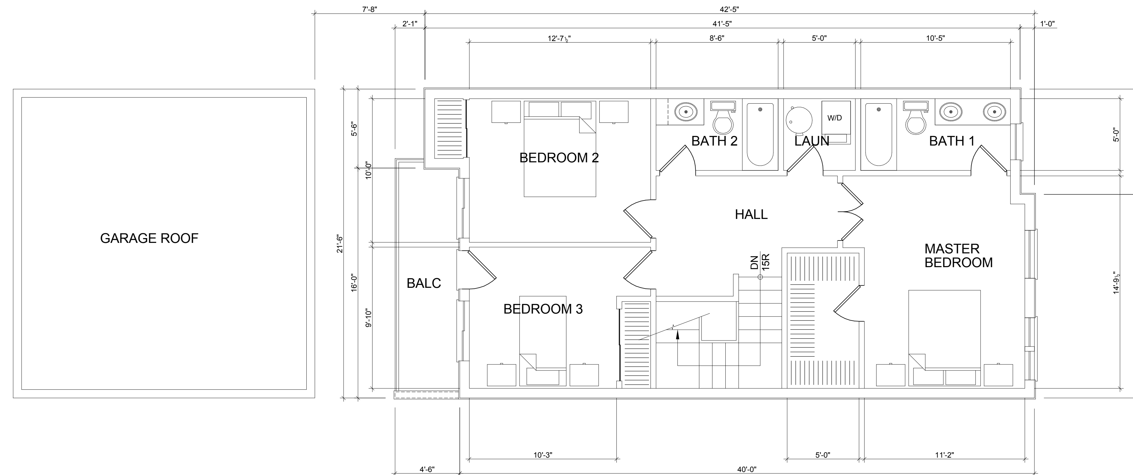
UNITS 1-7 - SECOND FLOOR PLAN
