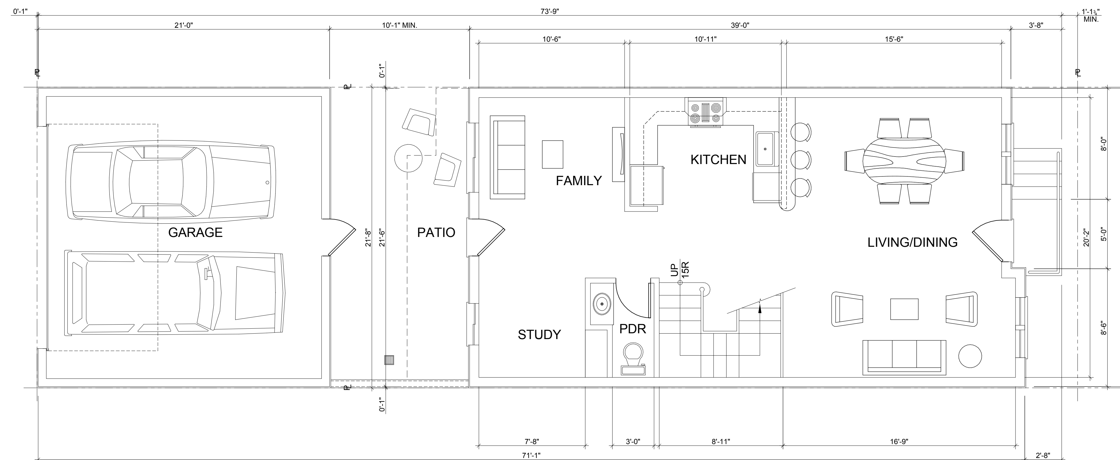
UNITS 1-7 - FIRST FLOOR PLAN
